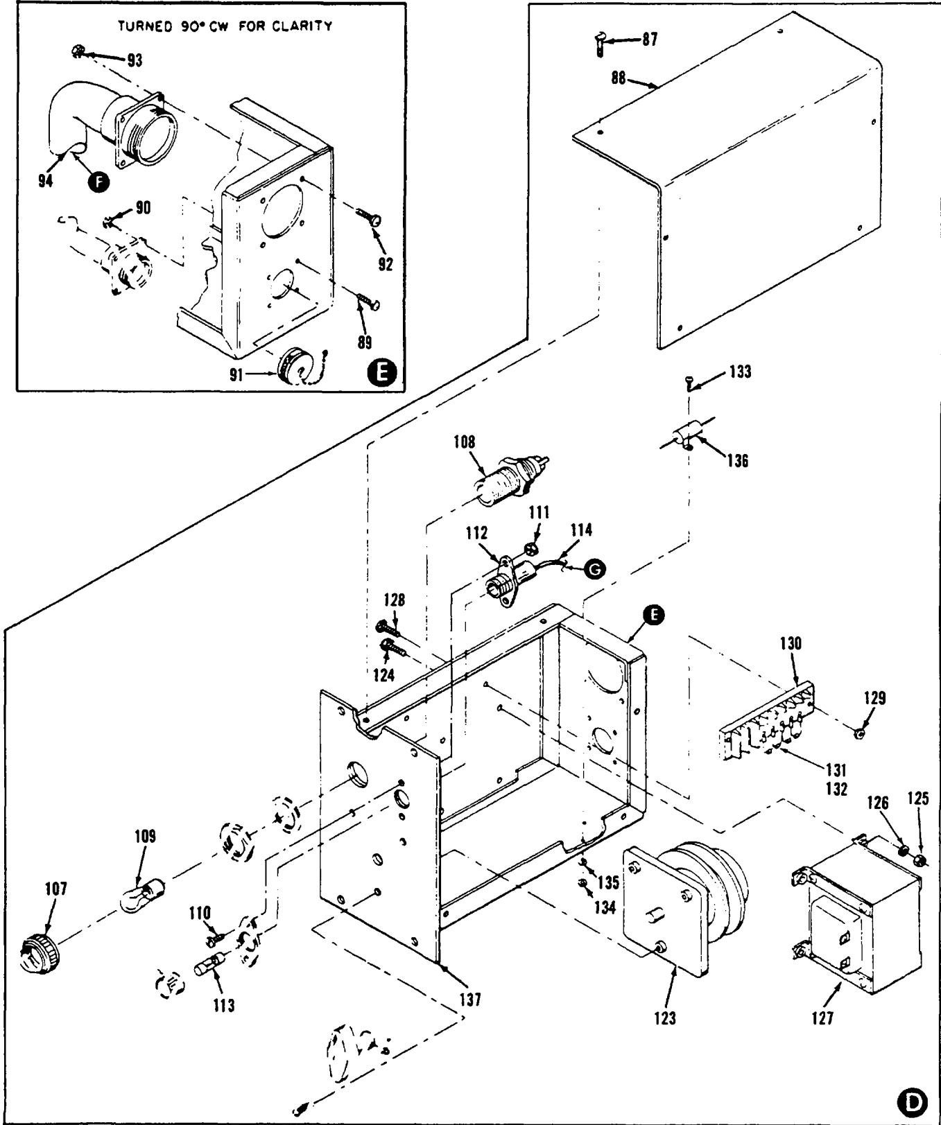
Figure 83. Electrical Winterization Kit (Sheet 5 of 6)
