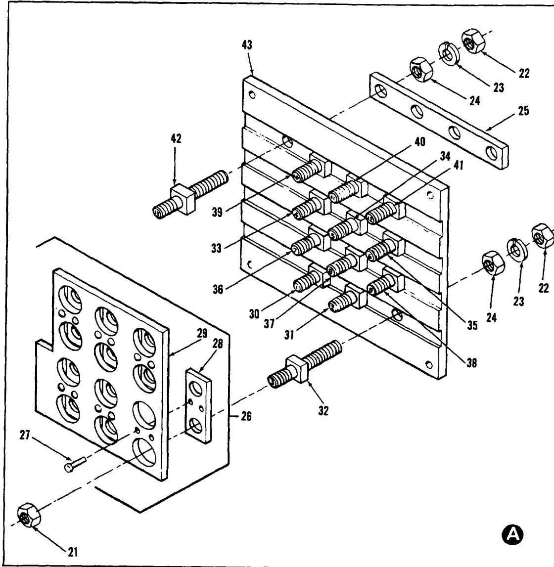
Figure 26. Reconnection Terminal Board Assembly and Related Parts (Sheet 2 of 2)
