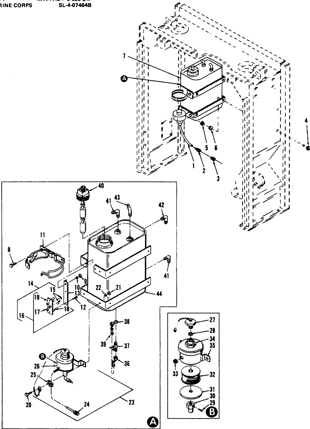
Figure 36. Day Tank, Ether Kit, and Related Parts
